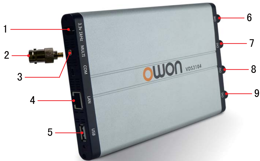
Figure 3-3 Ports of the Oscilloscope (take VDS3104(L) for instance)
